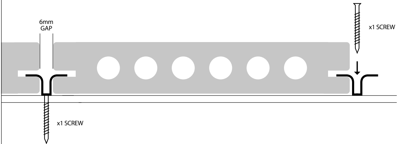
DECK FIXING CLIP
